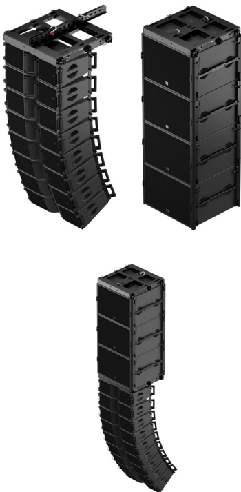
M-BUMP + M-BAR Flying and stacking frame up to 24 Kara II
