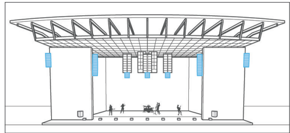
Shed Scene and Extension LISA Focus system with Kara II at 110°
